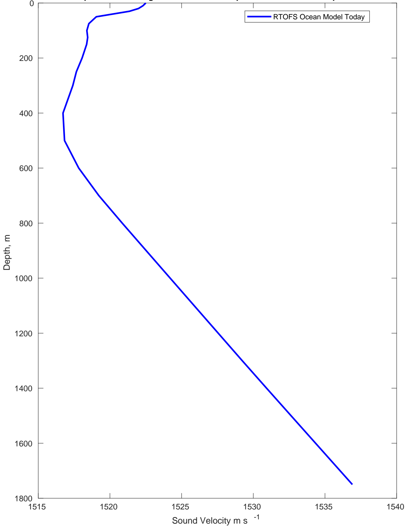
Sound Velocity Profile for Lighthouse Greece Pipeline-OSS1 on 24-Apr-2022 00:00:00
